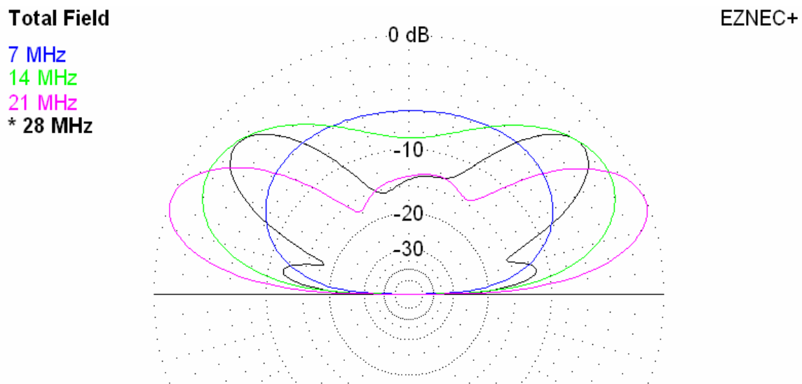
Figure 3: Far-field elevation patterns for the "Compact Quad"
