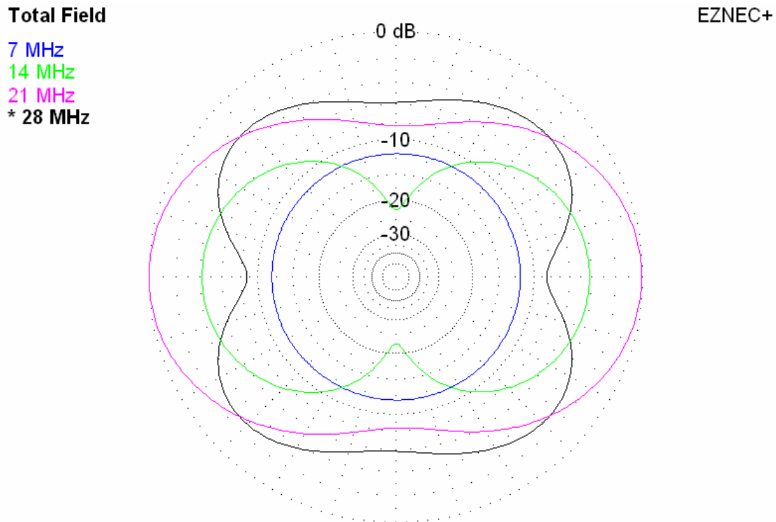
Figure 4 - Azimuth pattern for a takeoff angle of 10 degrees
